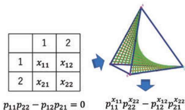
Many statistical models can be interpreted as algebraic varieties. Algebraic quantities can offer valuable insights for statistical inference.
